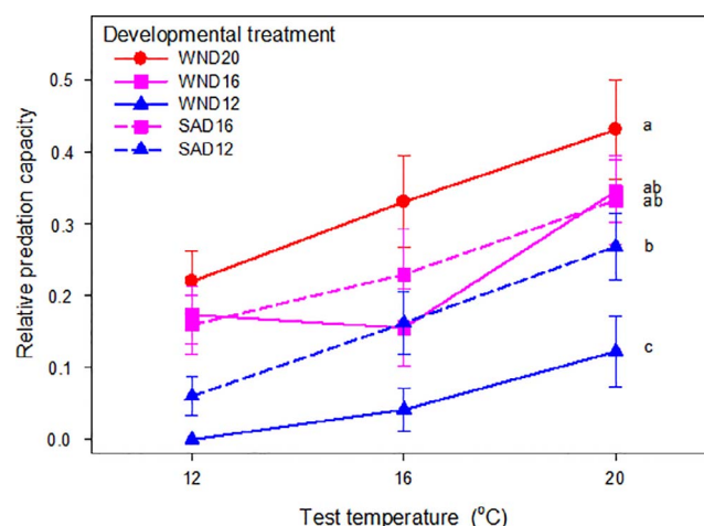
Fig. 1. Relative predation capacity (mean \pm SE) at different temperatures of O. majusculus females from different developmental temperature treatments. Treatment codes: WND20, WND16, WND12 = whole nymphal development at 20, 16, 12 °C; SAD16, SAD12 = subadult development at 16, 12 °C. Letters to the right: treatments with the same letter are not significantly different (multiple comparisons of ls-means using t -test with adjusted P -value (Holm method)). Sample sizes for each developmental treatment at test temperatures 12, 16, 20 °C, respectively: WND20: N = 19, 18, 17 ; WND16: N = 16, 16, 16 ; WND12: N = 9, 7, 8 ; SAD16: N = 16, 15, 15 ; SAD12: N = 14, 14, 14 .
